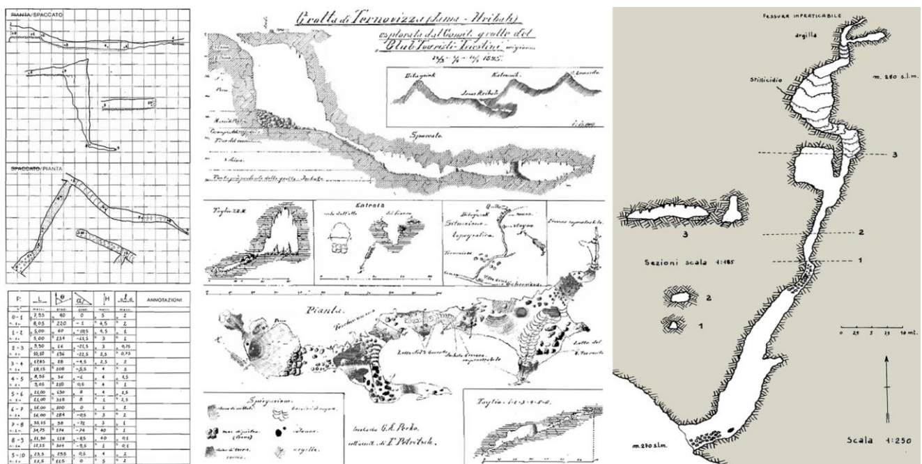
Fig. 1: The cave surveying - (from left to right) eidotypes and the field books, notes and sketches, final graphic rendering for the underground space (from the Manual of Hypogeum Surveying and the Teaching notebooks by the Italian Speleological Society).
